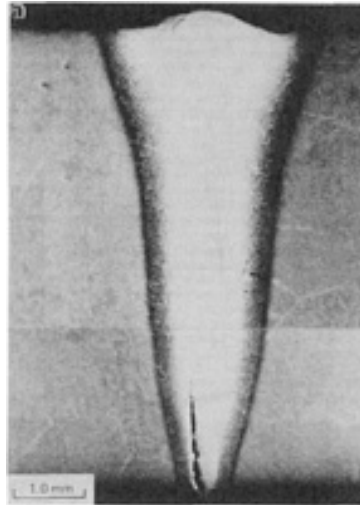
FIG. 3 CRACKING IN ALPHA-2 ELECTRON-BEAM WELD
