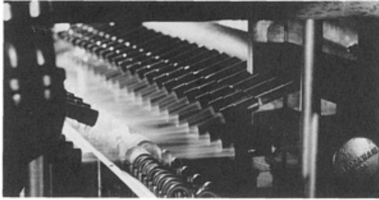
FIG. 1 AUTOMATED TORCH BRAZING SYSTEM
