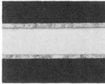
FIG. 1 PHOTOMICROGRAPH OF TYPICAL CLAD BRAZING MATERIAL, C12200 COPPER CLAD TO 304 L STAINLESS STEEL
