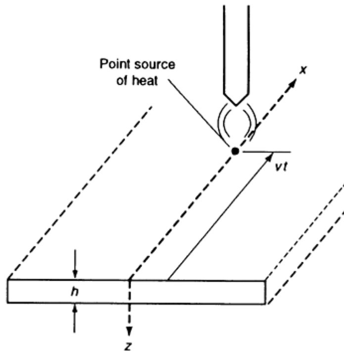
FIG. 1 MOVING POINT SOURCE IN INFINITE PLATE
