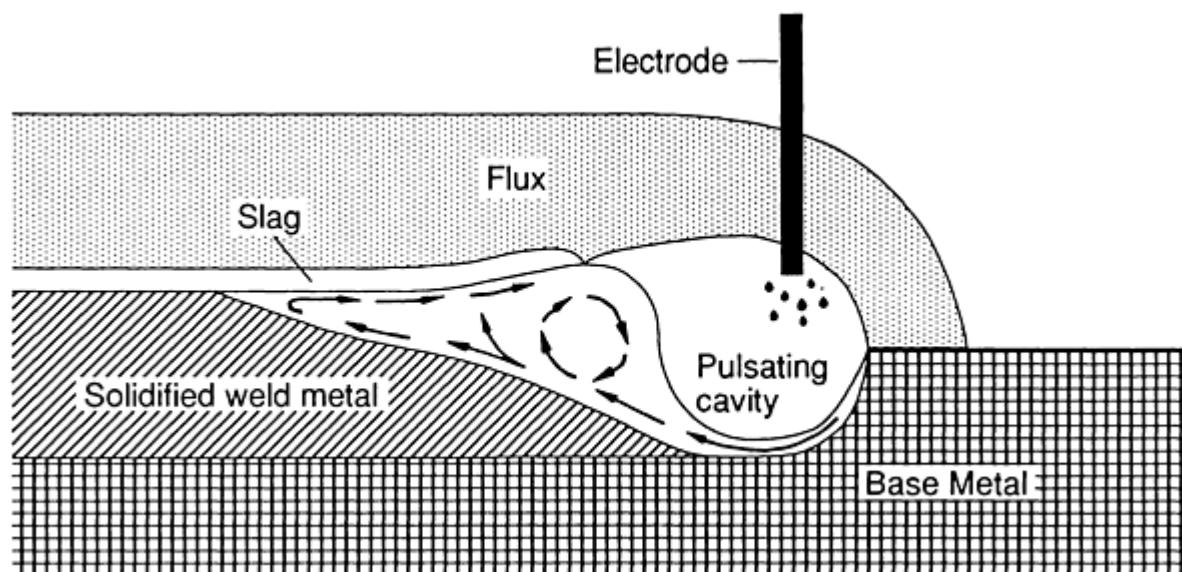
FIG. 12 SCHEMATIC SHOWING TYPICAL FLOW PATTERN IN A SUBMERGED ARC WELD POOL. SOURCE: REF 18
