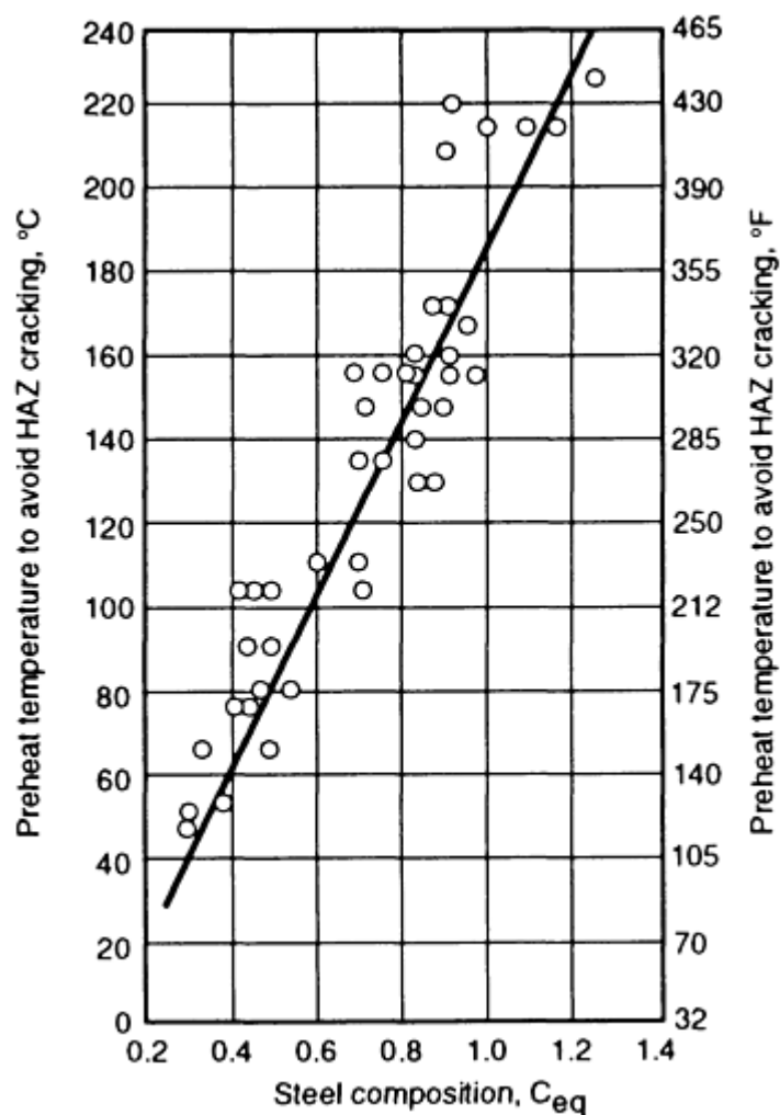
FIG. 5 CARBON EQUIVALENT VERSUS MINIMUM PREHEAT TEMPERATURE. THE BEST-FIT LINE SHOWN MAY BE REPRESENTED APPROXIMATELY BY: T = 210(C_{E0}) - 25 , WHERE T IS THE PREHEAT TEMPERATURE (°C).
