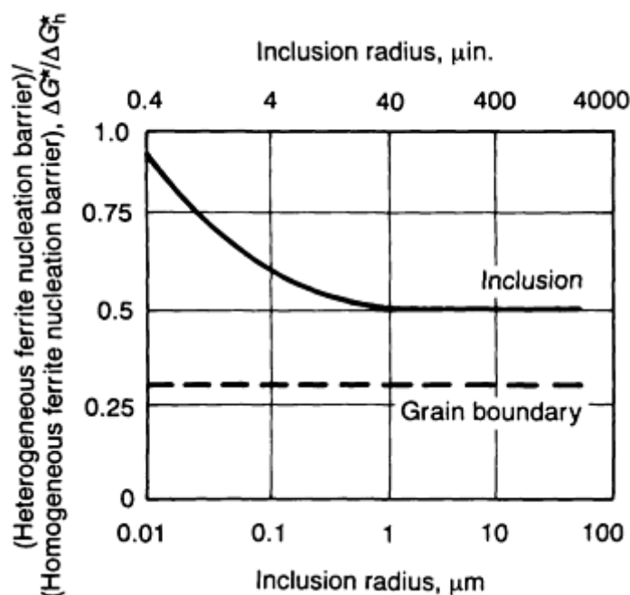
FIG. 17 EFFECT OF PARTICLE RADIUS ON ENERGY BARRIER TO FERRITE NUCLEATION AT INCLUSIONS, \Delta G^*_H (HETEROGENEOUS), NORMALIZED RELATIVE TO THE HOMOGENEOUS NUCLEATION BARRIER, \Delta G^*_H (HOMOGENEOUS). CORRESPONDING ENERGY BARRIER TO NUCLEATION OF FERRITE AT AUSTENITE GRAIN BOUNDARIES IS INDICATED BY HORIZONTAL BROKEN LINE. SOURCE: REF 6
