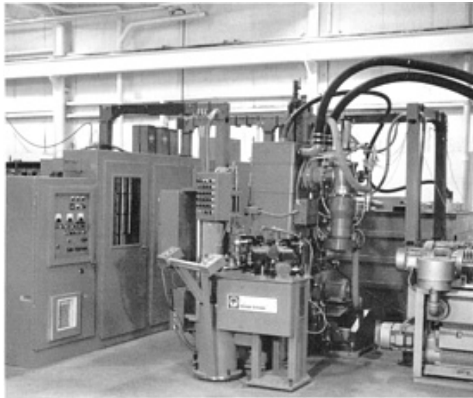
FIG. 10 STANDARD DIAL-INDEX TABLE-TYPE EBW-NV SYSTEM. COURTESY OF LEYBOLD-HERAEUS VACUUM SYSTEMS INC.
