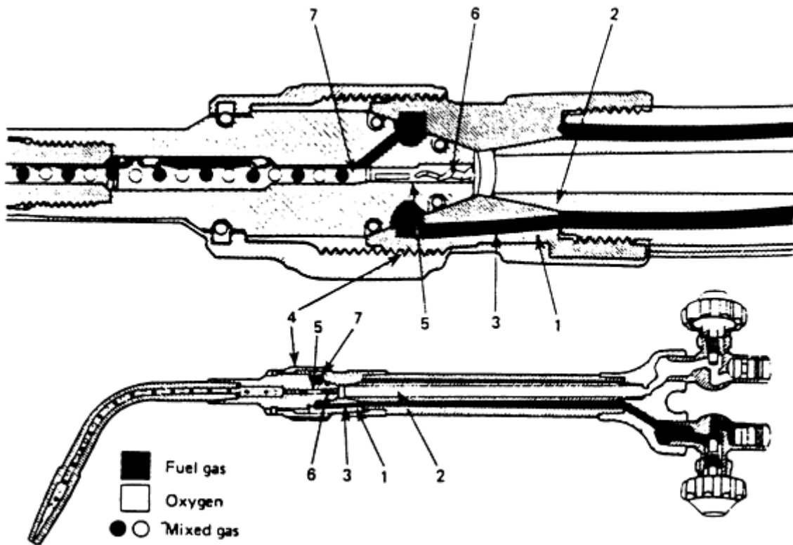
FIG. 4 SCHEMATIC SHOWING CROSS-SECTIONAL VIEW OF A SPIRAL EQUAL-PRESSURE MIXER. (1) WELDING TORCH HEAD. (2) OXYGEN TUBE FROM TORCH HEAD. (3) ACETYLENE (FUEL GAS) PASSAGES FROM TORCH HEAD. (4) NOZZLE NUT. (5) WELDING NOZZLE CONE END. (6) SPIRAL IN WELDING NOZZLE. (7) MIXER ORIFICE AND MIXING CHAMBER
