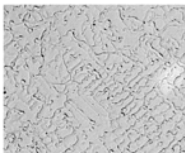
FIG. 1 TYPICAL WELD METAL MICROSTRUCTURE OF UHIMET ALLOY (UNS R31233) OBTAINED WITH GMAW DEPOSIT WHEN SHORT-CIRCUITING MODE OF TRANSFER IS USED. SAMPLE WAS ETCHED WITH HCL AND OXALIC ACID. 500×
