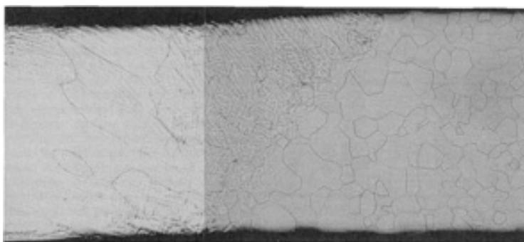
FIG. 2 MICROSTRUCTURE OF AS-WELDED GAS-TUNGSTEN ARC WELD IN BETA C SHEET
