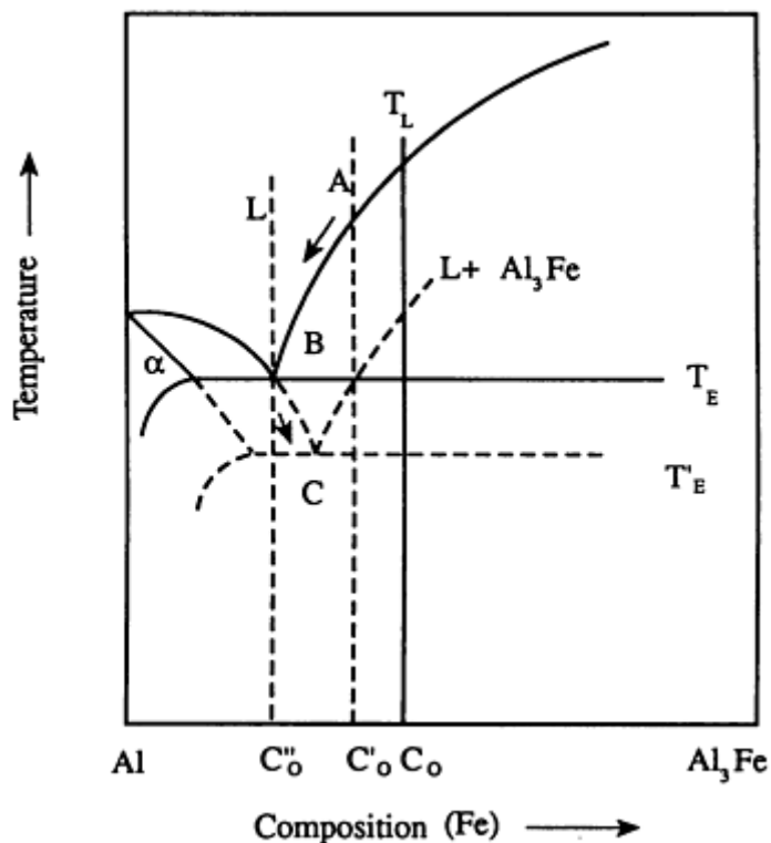
FIG. 6 AL-AL 3 FE PSEUDOBIINARY PHASE DIAGRAM ILLUSTRATING THE SEQUENCE OF SOLIDIFICATION EVENTS LEADING TO THE FORMATION OF TYPE A MICROSTRUCTURE. SOURCE: REF 20
