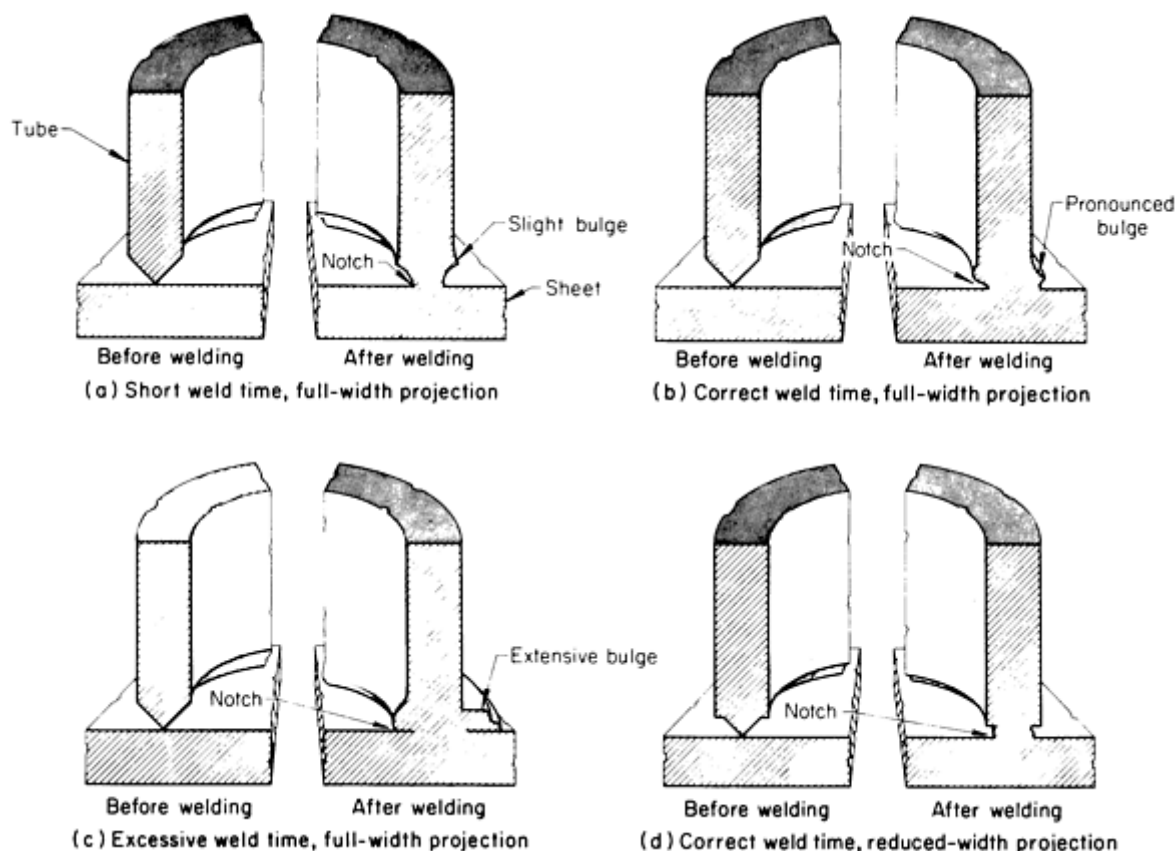
FIG. 6 CHARACTERISTICS OF PROJECTION COLLAPSE DURING ANNULAR PROJECTION WELDING WITH DIFFERENT BASE PROJECTION WIDTHS. (A) SHORT WELD TIME, FULL-WIDTH PROJECTION. (B) CORRECT WELD TIME, FULL-WIDTH PROJECTION. (C) EXCESSIVE WELD TIME, FULL-WIDTH PROJECTION. (D) CORRECT WELD TIME, REDUCED-WIDTH PROJECTION
