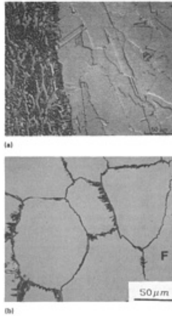
FIG. 9 MICROSTRUCTURES OF LASER-BEAM-WELDED AUSTENITIC STAINLESS STEELS. (A) GAS-TUNGSTEN ARC WELD SHOWN ON LEFT, WITH CO 2 LASER-BEAM WELD SHOWN ON RIGHT, IN ALLOY OF Cr_{Eq}/Ni_{Eq} = 1.8 . LASER-BEAM WELD ON RIGHT IS SINGLE-PHASE AUSTENITE FORMED AS A PRODUCT OF MASSIVE TRANSFORMATION. (B) FERRITIC STRUCTURE FORMED IN LASER-BEAM WELD OF Cr_{Eq}/Ni_{Eq} = 2.0 . SOURCE: REF 26, 27
