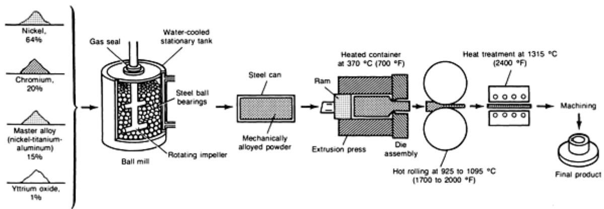
FIG. 1 SCHEMATIC SHOWING TYPICAL PROCESS OPERATIONS USED IN THE PRODUCTION OF MECHANICALLY ALLOYED OXIDE-DISPERSION-STRENGTHENED PRODUCTS
