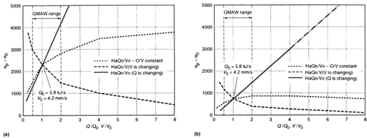
FIG. 7 PEAK TEMPERATURE DETERMINED BY THE POINT HEAT SOURCE SOLUTION. (A) AT 6.4 MM ( \frac{1}{4} IN.) FROM THE CENTER. (B) AT 13 MM ( \frac{1}{2} IN.) FROM THE CENTER
