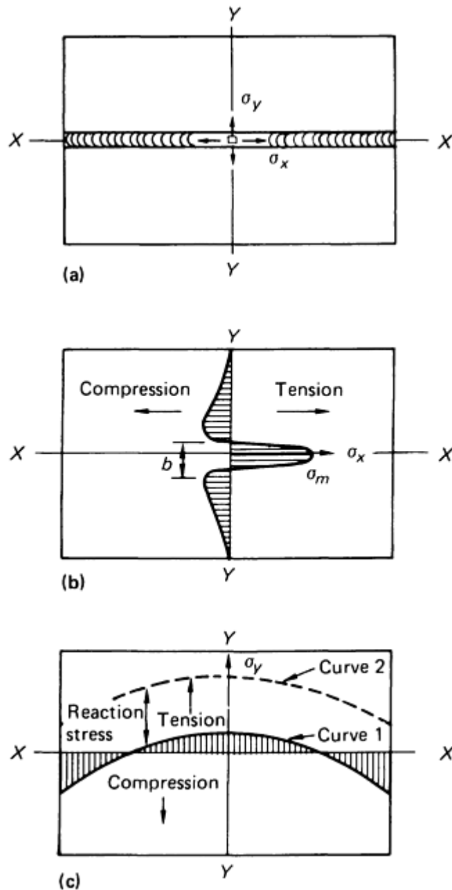
FIG. 3 TYPICAL DISTRIBUTIONS OF RESIDUAL STRESSES IN A GROOVE WELD. (A) GROOVE WELD. (B) DISTRIBUTION OF \sigma_x ALONG YY. (C) DISTRIBUTION OF \sigma_y ALONG XX. SOURCE: WELDING RESEARCH COUNCIL
