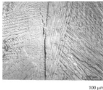
FIG. 8 SOLIDIFICATION CRACK IN ELECTRON-BEAM WELD ALONG WELD CENTER IN REGION WHERE SOLIDIFICATION OCCURRED AS PRIMARY AUSTENITE AS A RESULT OF HIGHER SOLIDIFICATION AND COOLING RATES
