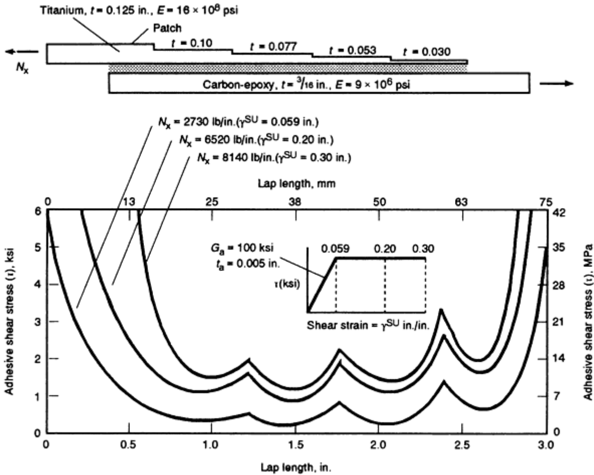
FIG. 6 THE EFFECT OF ADHESIVE PLASTICITY ON JOINT LOAD-CARRYING CAPABILITY. SEE FIG. 4 FOR EXPLANATION OF SYMBOLS. ORIGINAL SPECIMEN DIMENSIONS GIVEN IN INCHES
