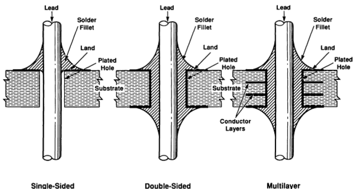
FIG. 8 SINGLE-SIDED, DOUBLE-SIDED, AND MULTILAYER SOLDER JOINT CONFIGURATIONS FOR THROUGH-HOLE TECHNOLOGY
