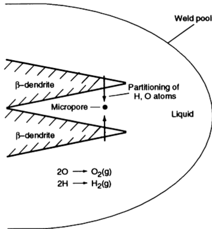
FIG. 16 SCHEMATIC DIAGRAM SHOWING HOW MICRO-PORES ARE NUCLEATED BETWEEN BETA-TITANIUM DENDRITES DURING WELD SOLIDIFICATION
