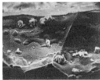
FIG. 6 INTERGRANULAR FRACTURE SURFACE SHOWING PARTIAL INTERGRANULAR WETTING WITH BOTH SOLID-SOLID AND LIQUID-LIQUID BONDING. 500×
