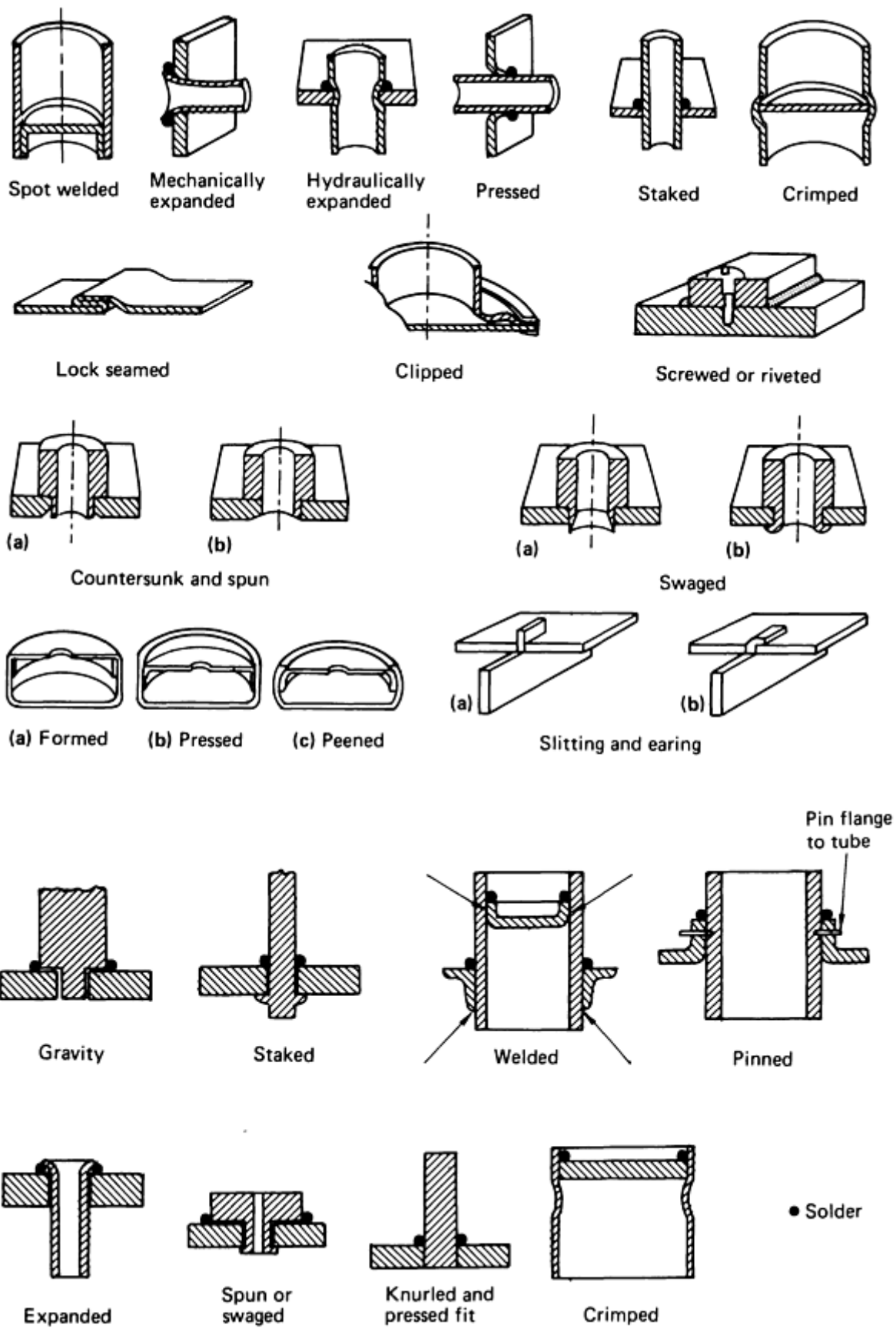
FIG. 21 SELF-JIGGING JOINT CONFIGURATIONS
