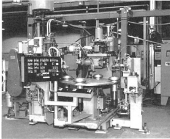
FIG. 8 CUSTOM-DESIGNED EBW-MW SYSTEM USED TO PRODUCE AUTOMOTIVE PARTS. COURTESY OF SCI AKY BROS., INC.
