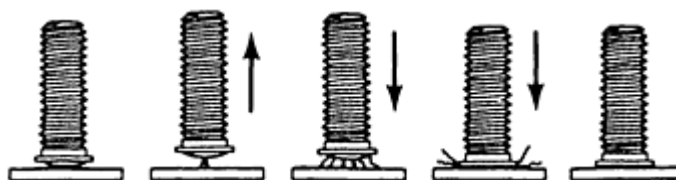
FIG. 4 DRAWN-ARC CD STUD WELDING. SEE TEXT FOR EXPLANATION. SOURCE: REF 1
