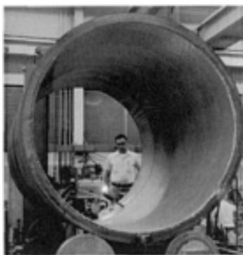
FIG. 29(A) WELD CLADDING OF A 1.8 M (6 FT) INNER DIAMETER PRESSURE VESSEL SHELL WITH 50 MM (2 IN.) WIDE, 0.64 MM (0.025 IN.) THICK STAINLESS STEEL STRIP. COURTESY OF J.J. BARGER, ABB COMBUSTION ENGINEERING
