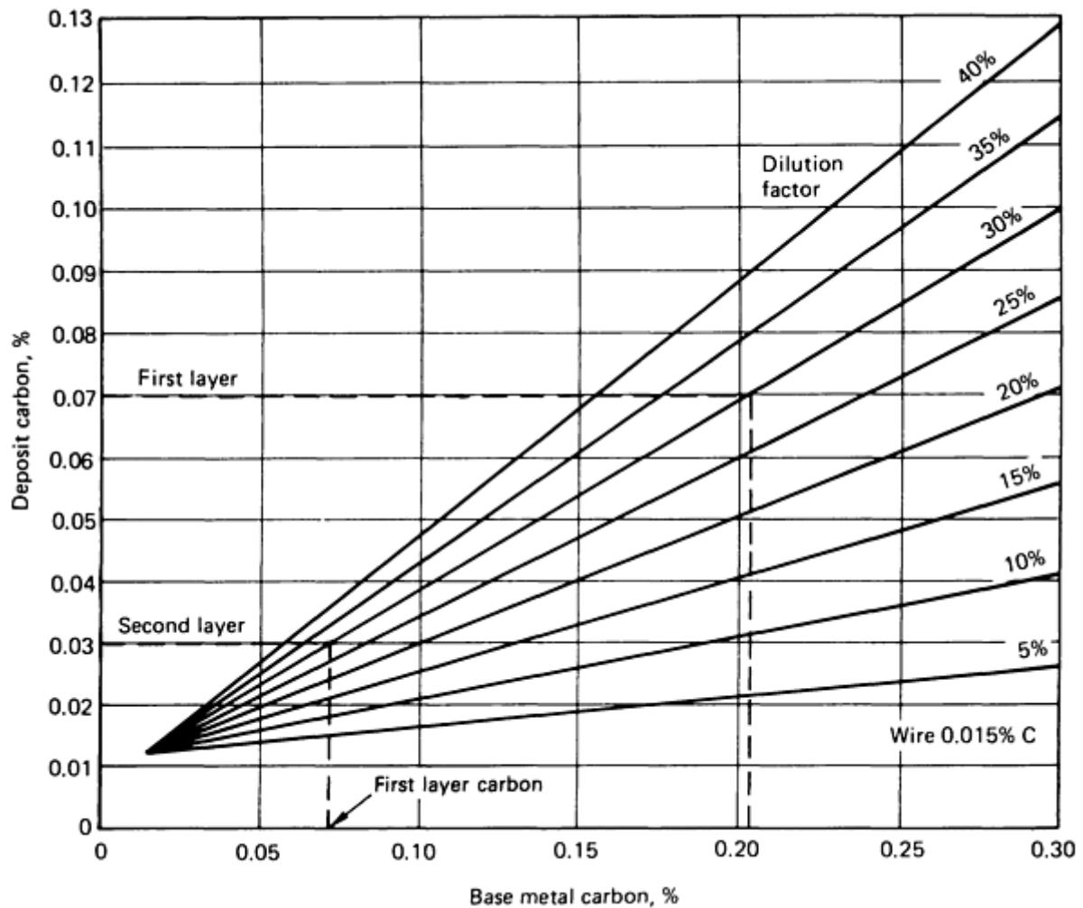
FIG. 24 PERCENTAGE OF CARBON IN THE DEPOSIT AFTER BASE METAL CARBON AND CLADDING DILUTION FACTORS HAVE BEEN ESTABLISHED. SOURCE: REF 26
