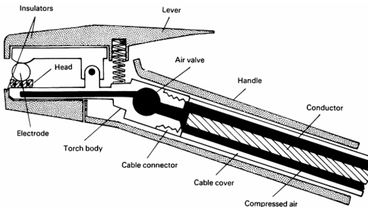
FIG. 3 CUTAWAY VIEW OF A MANUAL GOUGING TORCH WITH AIR FLOW ON BOTTOM OF ELECTRODE
