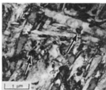
FIG. 11 TRANSMISSION ELECTRON MICROGRAPH OF LASER WELD FUSION ZONE IN RAPIDLY-SOLIDIFIED/POWDER METALLURGY TI-8AL-2.8SN-5.4HF-3.6TA-1Y-0.2SI ALLOY SHOWING YTTRIUM-ENRICHED DISPERSOIDS (INDICATED BY ARROWS) LOCATED ALONG SOLIDIFICATION SUBSTRUCTURE BOUNDARIES. SOURCE: REF 17
