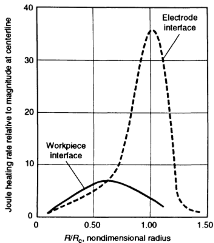
FIG. 10 JOULE HEATING RATE RATIO VERSUS NONDIMENSIONAL RADIUS. TIME, 2 CYCLES; R_c , RADIUS OF CONTACT. SOURCE: REF 27
