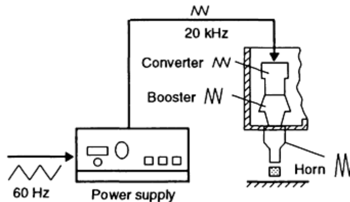
FIG. 11 SCHEMATIC OF ULTRASONIC-WELDING COMPONENTS
