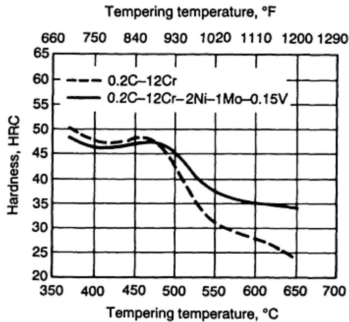
FIG. 11 TEMPERING RESPONSE (2 H AT TEMPERATURE) OF TYPES 420 AND MODIFIED 420 CONTINUOUS CASTER ROLL OVERLAY. SOURCE: REF 16
