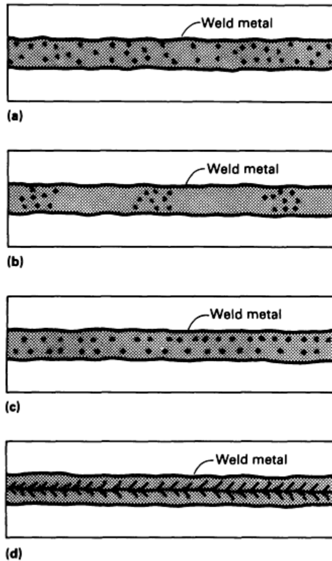
FIG. 1 TYPES OF GAS POROSITY COMMONLY FOUND IN WELD METAL. (A) UNIFORMLY SCATTERED POROSITY. (B) CLUSTER POROSITY. (C) LINEAR POROSITY. (D) ELONGATED POROSITY
