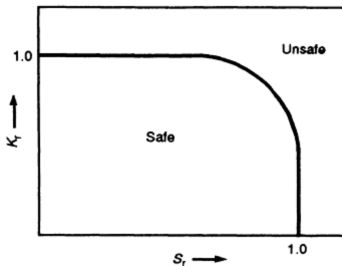
FIG. 4 BASIC CONCEPT OF FAILURE-ASSESSMENT DIAGRAM
