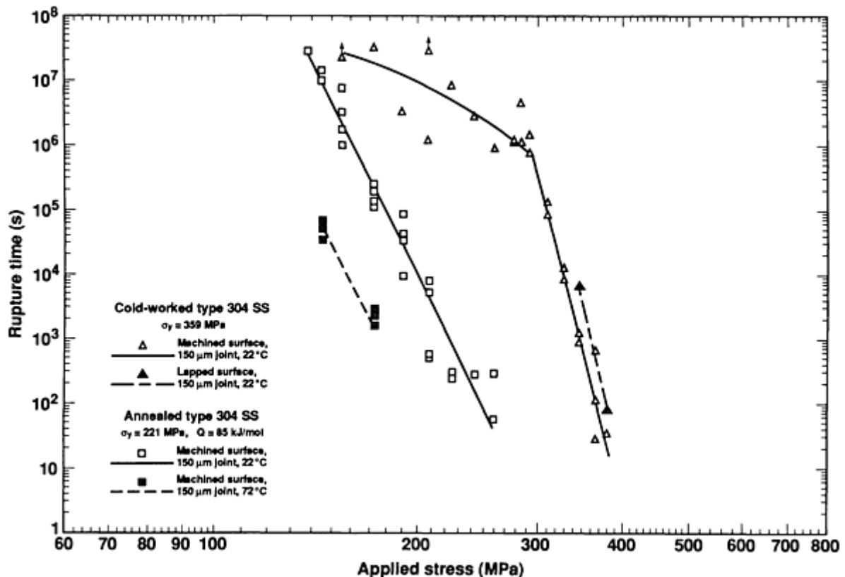
FIG. 7 CREEP-RUPTURE BEHAVIOR OF SOLID-STATE-WELDED SILVER INTERLAYERS ( T/D = 0.024 ) JOINING ONE OF TWO DIFFERENT STRENGTHS OF TYPE 304 STAINLESS STEEL BASE METALS (ANNEALED OR COLD-WORKED), BOTH OF WHICH UNDERGO TIME-DEPENDENT PLASTICITY OR CREEP AT AMBIENT TEMPERATURES AT STRESSES LESS THAN THE CONVENTIONAL YIELD STRESS OF THE METAL
