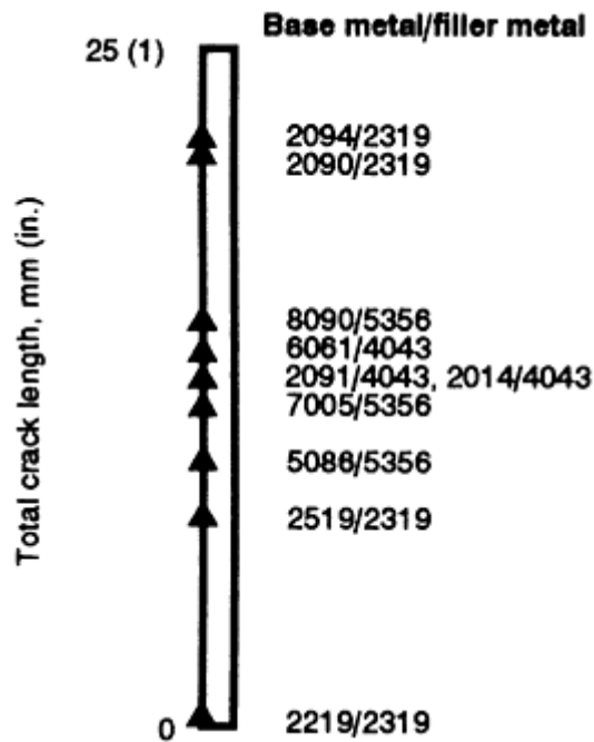
FIG. 3 TRANS-VARESTRAINT WELDABILITY DATA FOR ALUMINUM ALLOYS. SOURCE: REF 25
