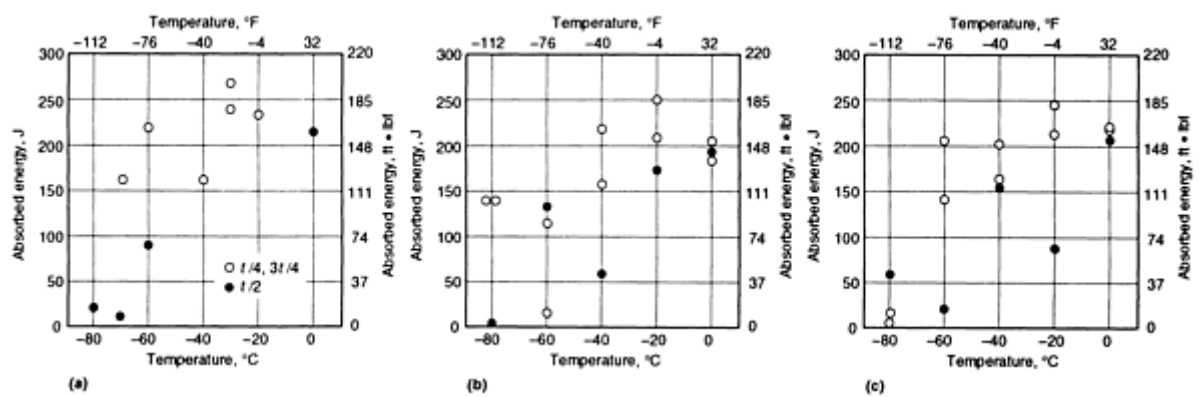
FIG. 10 EFFECT OF MULTIPLE PWHT CYCLES ON THE HAZ CHARPY V-NOTCH PROPERTIES OF A CARBON-MANGANESE GRADE STEEL. (A) WELD 1; PWHT, 1 × 2H. (B) WELD 2; PWHT, 2 × 2H. (C) WELD 3; PWHT, 3 × 2H. SOURCE: REF 25
