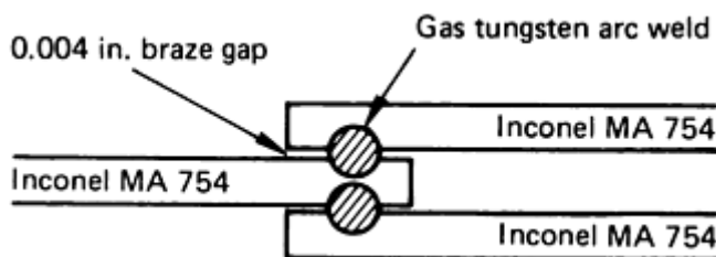
FIG. 4 BRAZING SPECIMEN ASSEMBLY USED TO EVALUATE STRESS-RUPTURE PROPERTIES OF BRAZED INCONEL MA 754
