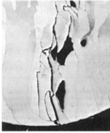
FIG. 13 INTERGRANULAR CORROSION OF A CONTAMINATED E-BRITE STAINLESS STEEL WELD. ELECTROLYTICALLY ETCHED WITH 10% OXALIC ACID. 200×. SOURCE: REF 47
