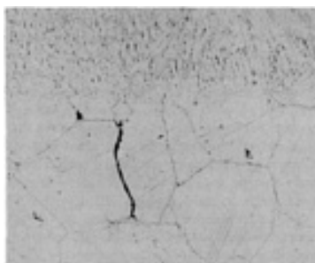
FIG. 1 PHOTOMICROGRAPH SHOWING A HEAT-AFFECTED ZONE MICROFISSURE IN A NICKEL-CHROMIUM ALLOY. SPECIMEN IS A GMAW 44.4 MM (1.75 IN.) PLATE. ELECTROLYTIC PHOSPHORIC ACID ETCHANT, 75×
