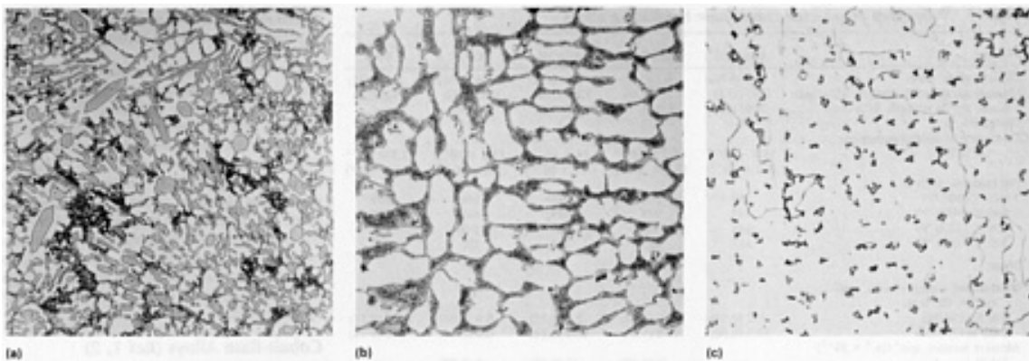
FIG. 5 MICROSTRUCTURES OF TWO-LAYER PLASMA TRANSFERRED ARC DEPOSIT CARBIDE-CONTAINING COBALT-BASE HARDFACING ALLOYS. (A) ERCOCR-C. (B) ERCOCR-A. (C) ERCOCR-E. 425 \times . SOURCE: REF 2
