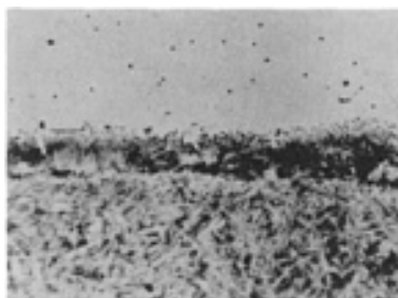
FIG. 2 PHOTOMICROGRAPH SHOWING WELD INTERFACE CROSS SECTION OF 0.81 MM (0.032 IN.) THICK HIGH-CARBON (0.9 WT% C) STEEL ULTRASONICALLY WELDED TO 0.81 MM (0.032 IN.) THICK IRON. 1000×
