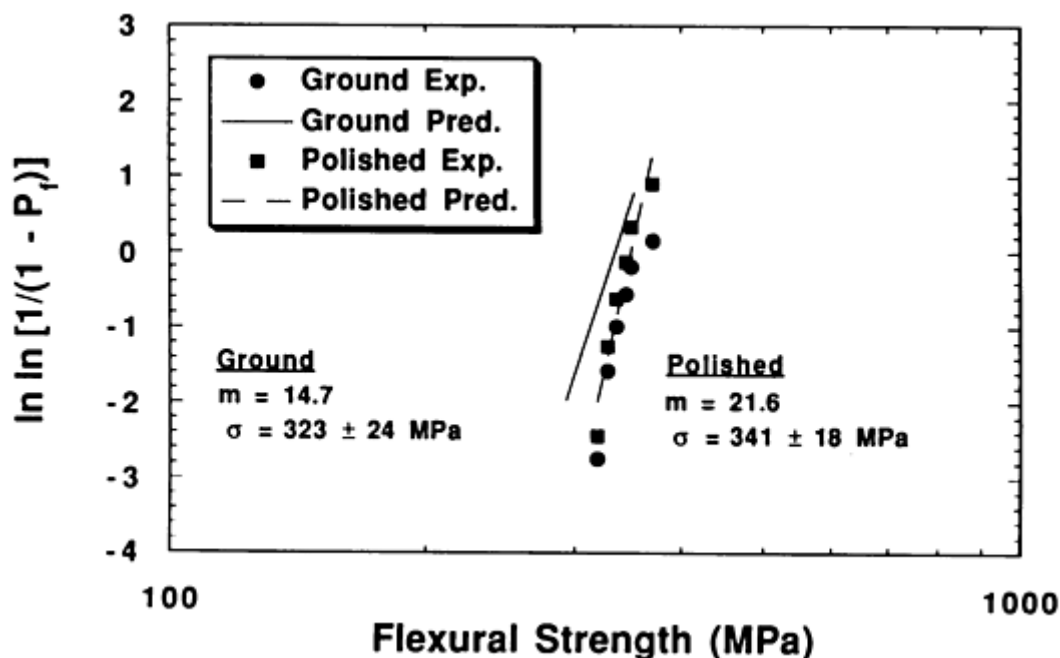
FIG. 2 EFFECT OF POLISHING INTERFACIAL AREA ON STRENGTH OF CU-41AG-3.5SN-7TI, AT.%, BRAZEMENT IN MCDANEL AD-998 ALUMINA
