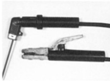
FIG. 3 SMAW ELECTRODE HOLDERS
