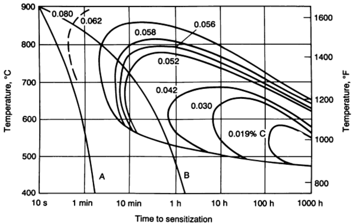
FIG. 6 TIME-TEMPERATURE-SENSITIZATION CURVES FOR TYPE 304 STAINLESS STEEL IN A MIXTURE OF \text{CuSO}_4 AND \text{HSO}_4 CONTAINING COPPER. SOURCE: REF 15. CURVES A AND B INDICATE HIGH AND MEDIUM COOLING RATES, RESPECTIVELY.
