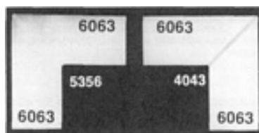
FIG. 7 CLEAR ANODIC COATING ON 6063 WELDS MADE WITH ALUMINUM-MAGNESIUM (5356) AND ALUMINUM-SILICON (4043) FILLERS
