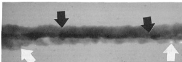
FIG. 7 RADIOGRAPH SHOWING POSITIVE IMAGE OF MACROSCOPICALLY VISIBLE DEFECTS IN THE X-65 PIPE STEEL OF FIG. 6. SEE FIG. 6 FOR DESIGNATION OF SPECIFIC DEFECTS.
