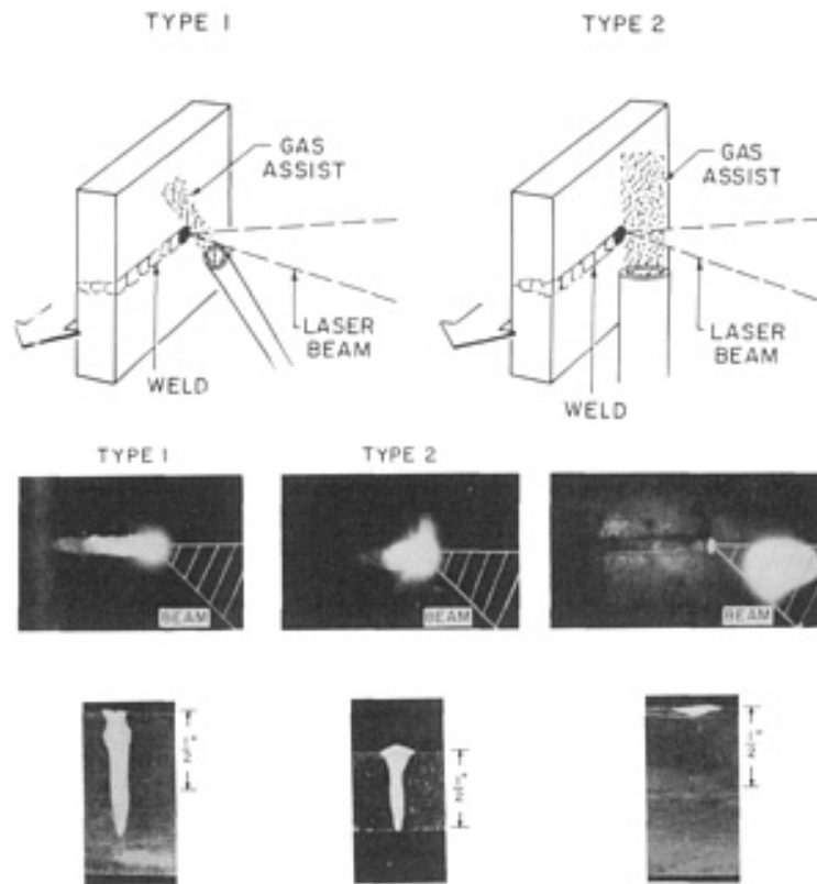
FIG. 5 EFFECT OF GAS ASSIST ON THE CROSS SECTION OF THE WELD. SOURCE: REF 18
