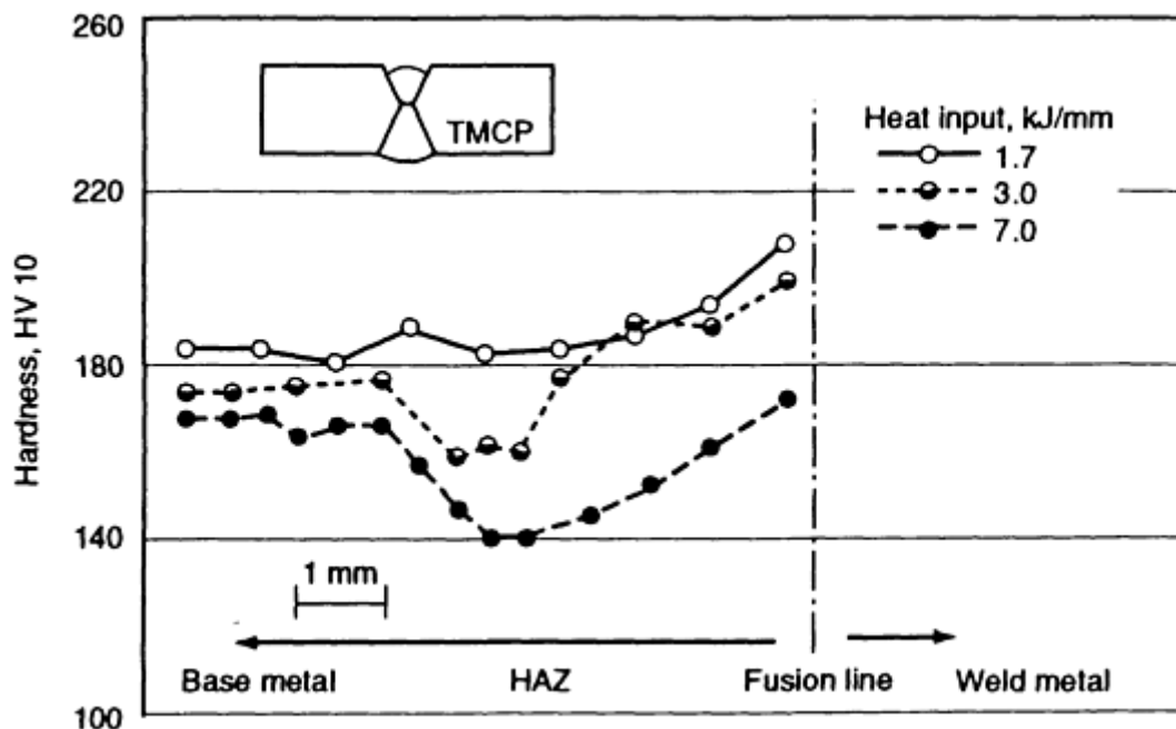
FIG. 7 VARIATION OF HARDNESS PROFILES IN HAZ OF TMCP STEEL WELDED WITH HEAT INPUT OF 1.7, 3.0, AND 7.0 KJ/MM (43, 76, AND 178 KJ/IN.). CARBON, 0.06%; SILICON, 0.14%; MANGANESE, 1.33%; PHOSPHORUS, 0.010%; SULFUR, 0.001%; COPPER, 0.31%; NICKEL, 0.31%; CHROMIUM, 0.05%; NIOBIUM, 0.15%; AND ALUMINUM, 0.034%. SOURCE: REF 13
