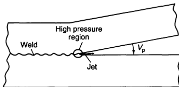
FIG. 5 JET FORMATION AT THE COLLISION POINT TO GENERATE WELD DURING EXW
