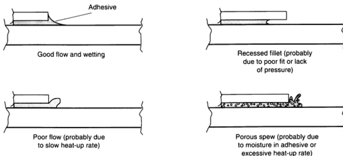
FIG. 5 EXAMPLES OF GOOD AND BAD ADHESIVE FILLETS
