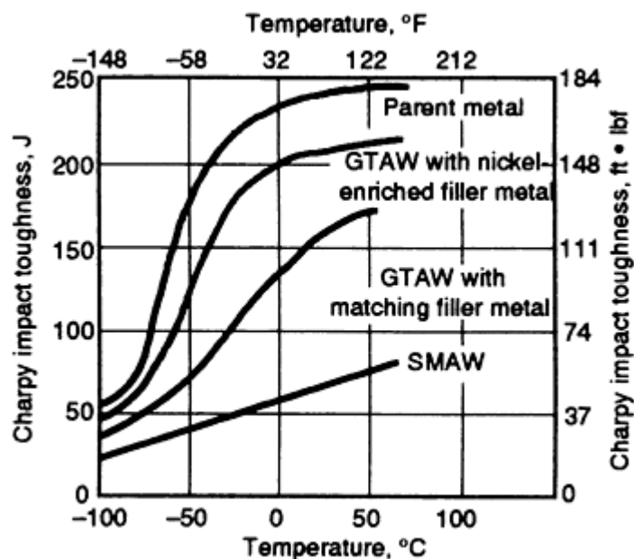
FIG. 4 PLOT OF CHARPY IMPACT TOUGHNESS VERSUS TEMPERATURE FOR FE-22CR-5.5NI-3MO-0.15N DSS BASE METAL AND WELDS PRODUCED WITH GAS-TUNGSTEN ARC WELDING (GTAW) AND SHIELDED METAL ARC WELDING (SMAW) PROCESSES. SOURCE: REF 2
