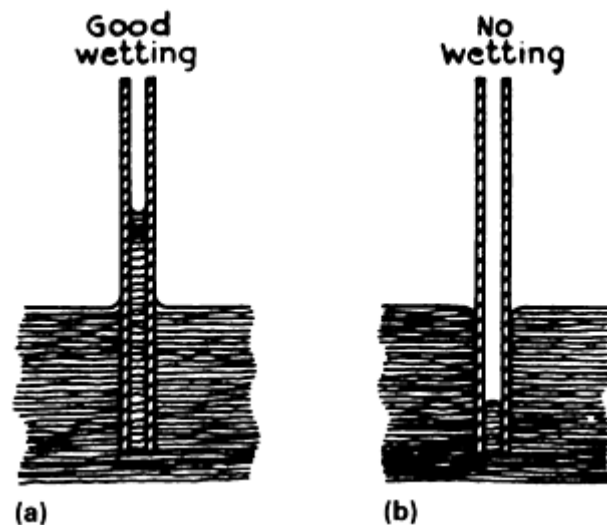
FIG. 1 SCHEMATIC SHOWING PRINCIPLE OF CAPILLARY ATTRACTION FOR SELECTED LIQUIDS WHEN THE LIQUID IS SANDWICHED BETWEEN TWO CLEAN GLASS PLATES. (A) WHEN IMMERSED IN WATER OR INK, A COLUMN WILL RISE BETWEEN THE PLATES BECAUSE OF WETTING. (B) WHEN THE PLATES ARE IMMERSED IN MERCURY, NO WETTING OCCURS AND THE COLUMN IS DEPRESSED. IF PARAFFIN PLATES ARE USED IN PLACE OF THE GLASS PLATES, IMMERSION OF THE PLATES IN MERCURY WILL PRODUCE WETTING.
