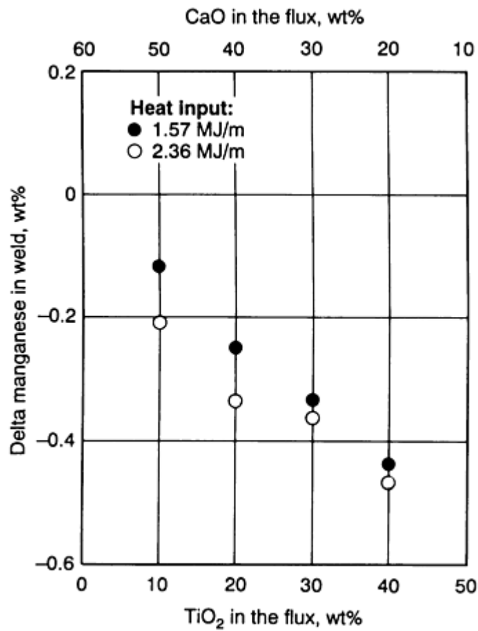
FIG. 3 PLOT OF CHANGES IN MANGANESE CONTENT IN THE WELD VERSUS THE VARIATION IN FLUX COMPOSITION AS A FUNCTION OF TWO-HEAT INPUTS. THE \text{SiO}_2 CONTENT WAS MAINTAINED AT 40% THROUGHOUT THE FLUX-CORED ARC WELDING PROCESS. SOURCE: REF 21
