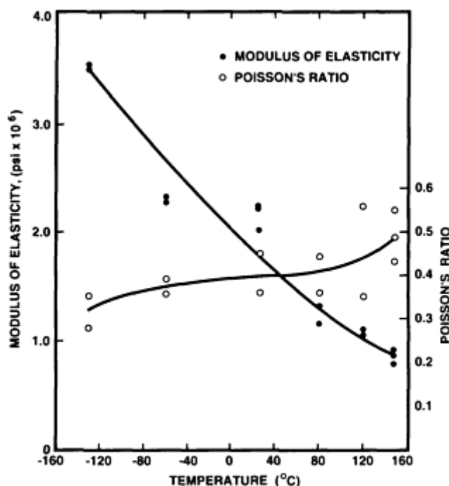
FIG. 9 TEMPERATURE DEPENDENCE OF TENSILE MODULUS AND POISSON'S RATIO OF 63SN-37PB SOLDER. SOURCE: REF 14
