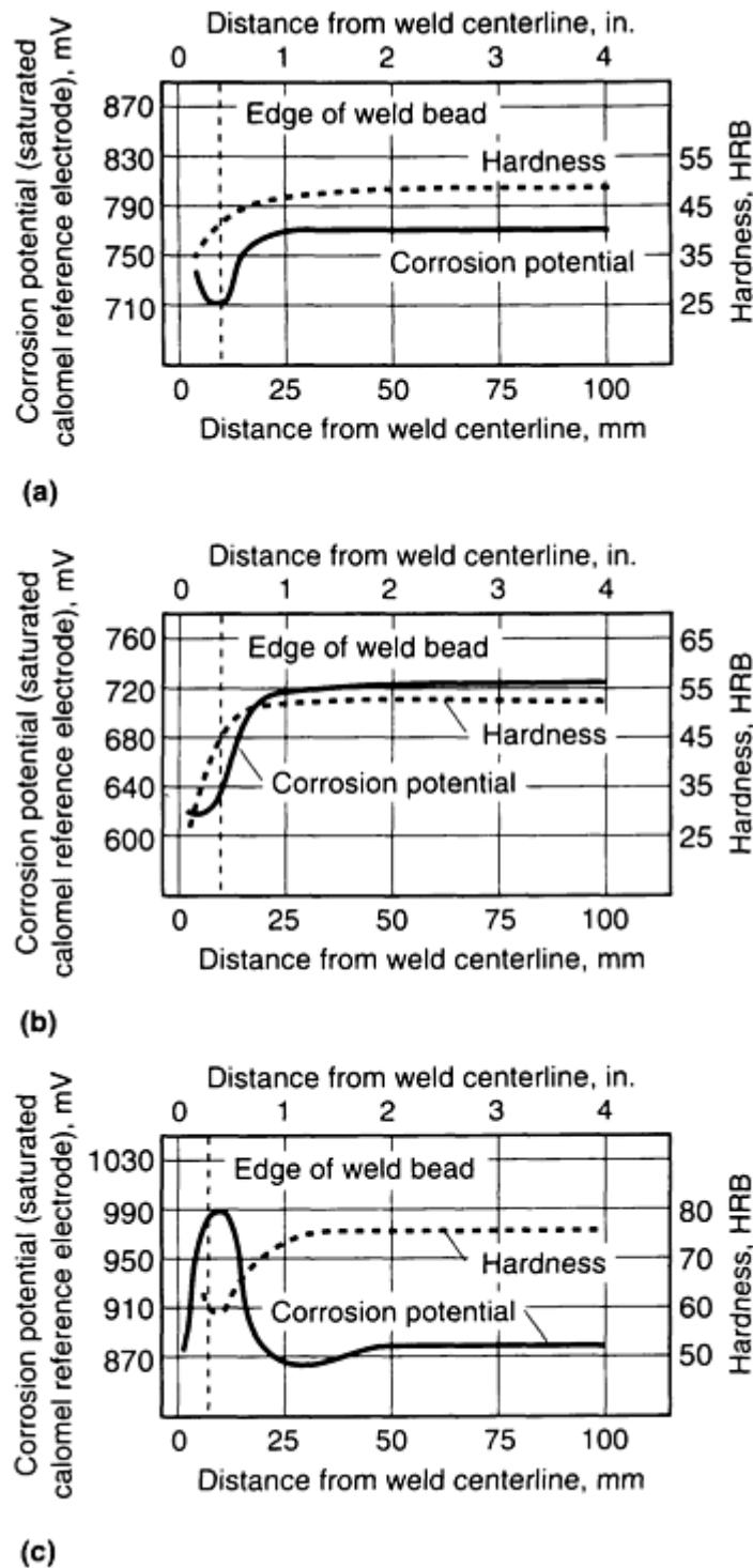
FIG. 13 PLOT OF CORROSION POTENTIAL AND HARDNESS LEVELS VERSUS DISTANCE FROM WELD CENTERLINE FOR SELECTED ALUMINUM ALLOYS. (A) ALLOY 5456-H321 (5556 FILLER METAL; DCRP-MIG WELD PRODUCED IN THREE PASSES). (B) 2219-T87 (2319 FILLER METAL; DCSP-TIG WELD PRODUCED IN TWO PASSES). (C) 7039-T651 (5183 FILLER METAL; DCRP-TIG WELD PRODUCED IN TWO PASSES). DCRP, DIRECT CURRENT REVERSE POLARITY; DCSP, DIRECT CURRENT STRAIGHT POLARITY. COURTESY OF ALCOA LABORATORIES
